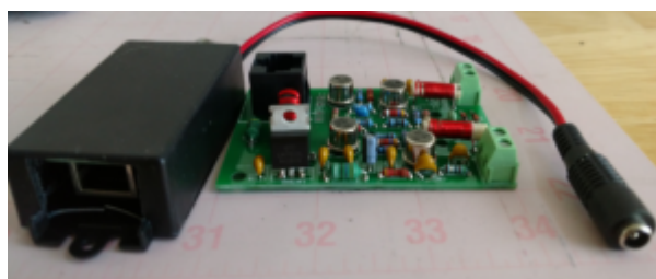
LNA & Balun/Power inserter boards.
